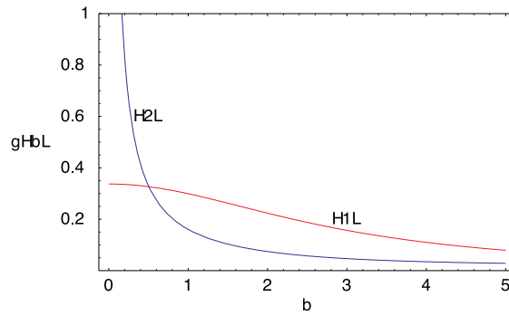
Figure 2. Marginal probability distribution of quantum Jeffreys prior for the temperature parameter, \beta with \beta_0 = 5 . Curve (1) refers to the distribution for the displaced squeezed state and curve (2) refers to the distribution for the undisplaced squeezed state. Note that whereas the marginal distribution for the undisplaced squeezed states (curve 2) tends to infinity as \beta \rightarrow 0 (high temperature), the distribution for the displaced squeezed states (curve 1) goes to a finite value in the same limit.
